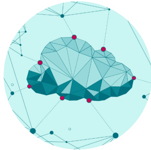
Machine Learning
